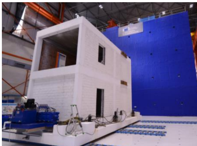
Figure 5. iRESIST+ experimental prototype at JRC’s European Laboratory for Structural Assessment (ELSA)
