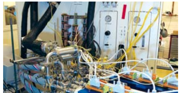
Fuel cell stack undergoing testing in the Petten facility
