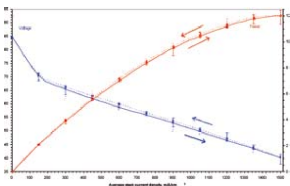
Figure 2: Polarisation curves (voltage/power vs. current density) of a PEFC stack of 11 kW nominal power output. The blue curves represent the average stack voltage during stepwise increase (solid line) and decrease (dotted line) of the stack current density while the red curves represent that of the corresponding average stack power. The error bars indicate the variations between maximum and minimum of these values
