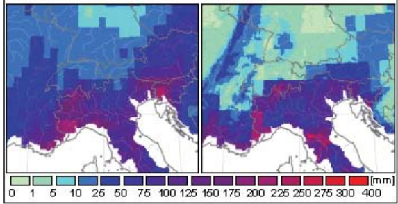
ECMWF 2004102812 10-day accumulated rainfall
