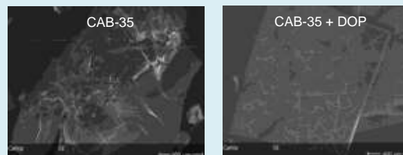
Figure 4. Different crack sizes formed in CAB films without and with DOP additive.
