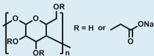
Figure 6. CMC is made of repeating anhydroglucose units, it contains carboxymethyl instead of acetyl or butyryl side groups.
