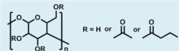
Figure 2. CAB is built up from repeating anhydroglucose units. Certain percentage of the –OH groups are converted to acetyl or butyryl groups.
