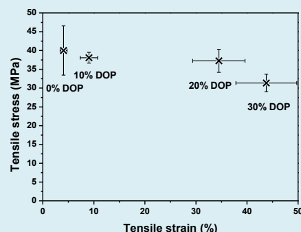
Figure 3. Stress-strain data of CAB films with different DOP content.
