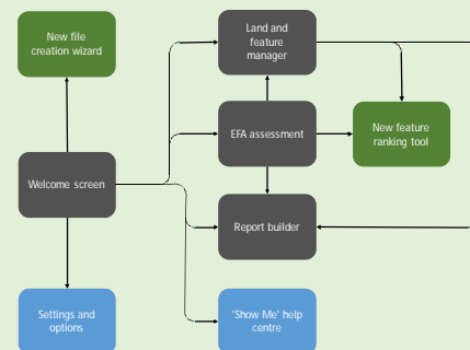
The structure of the EFA software interface
